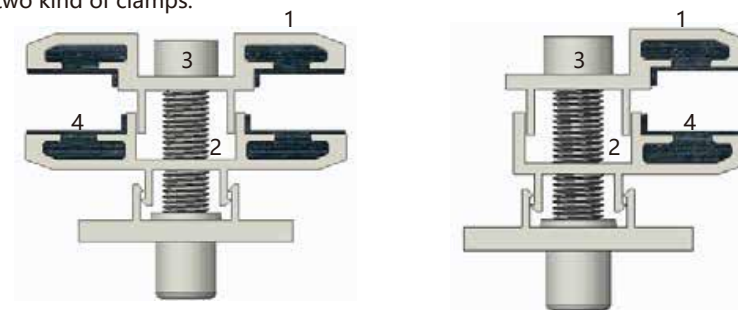
Figure 1 Double-side clamp
